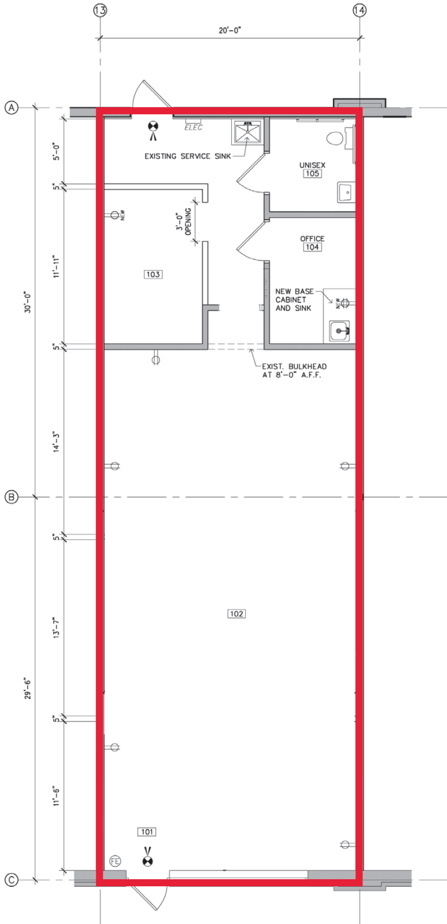
1 FLOOR PLAN LH1 SCALE: 1/4" = 1'-0"
